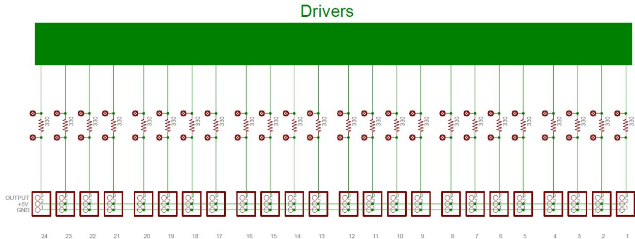
Figure 2-1. Signal Board Connector Wiring Diagram
